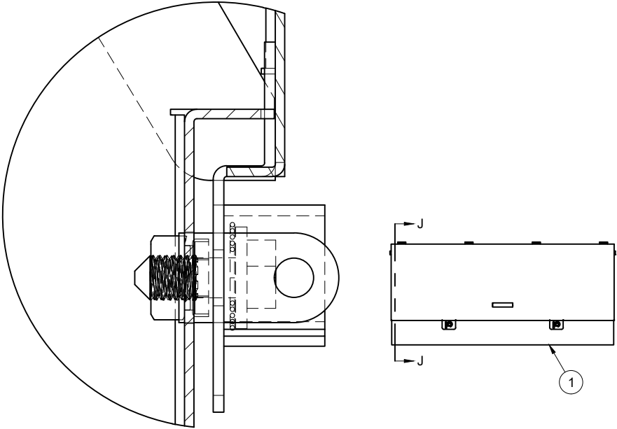
DETAIL N SCALE 1:1.5
